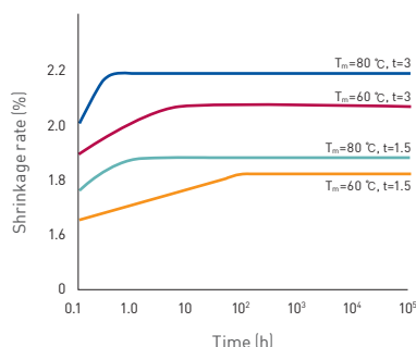
Fig 2-8. Shrinkage rate changes with mold temperature and specimen's thickness
