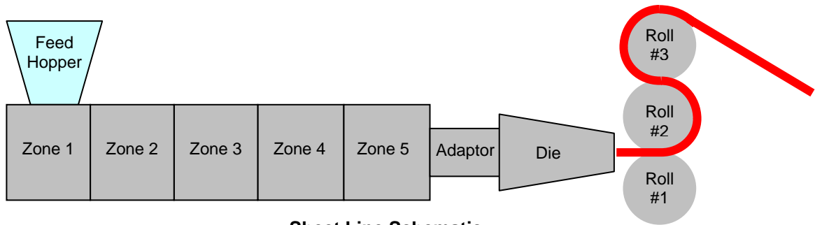
Sheet Line Schematic
