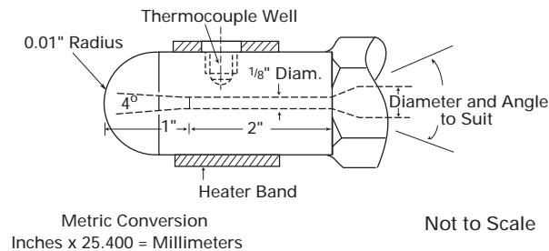
Figure 4. Nozzle (with reverse taper) Recommended for Molding
