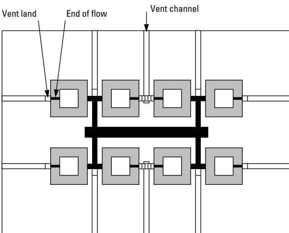
Fig. 4.11 Vent geometries ejector
