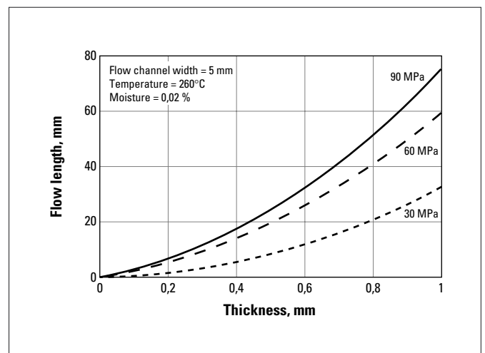
Fig. a.12 CRASTIN® SK609 NC010
