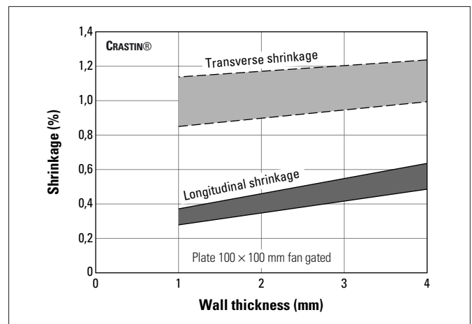
Fig 5.4 Shrinkage of 30% glass-fibre reinforced CRASTIN® types (e.g. SK605, SK645FR) as a function of wall thickness
