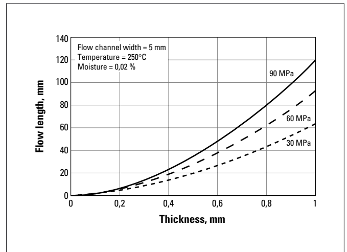
Fig. a.10 CRASTIN® SK605 NC010
