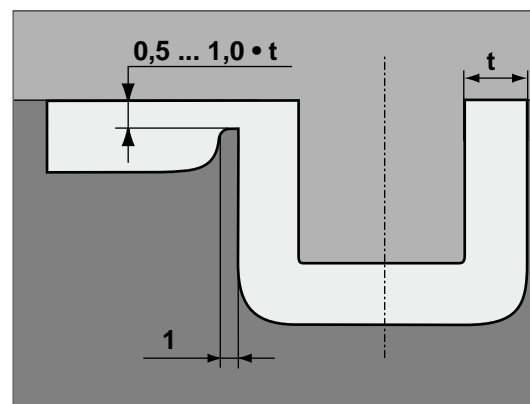
Fig. 4.8 Direct gate
