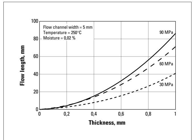
Fig. a.34 CRASTIN® SK645FR NC010
