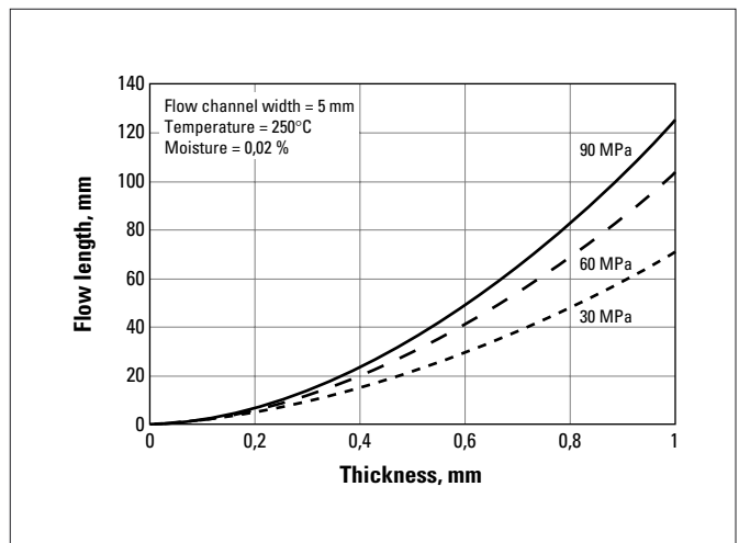
Fig. a.6 CRASTIN® S620F20 NC010
