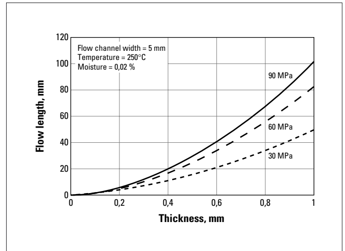
Fig. a.32 CRASTIN® SK642FR NC010
