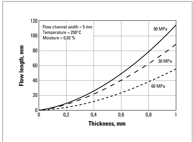
Fig. a.4 CRASTIN® S600F30 NC010
