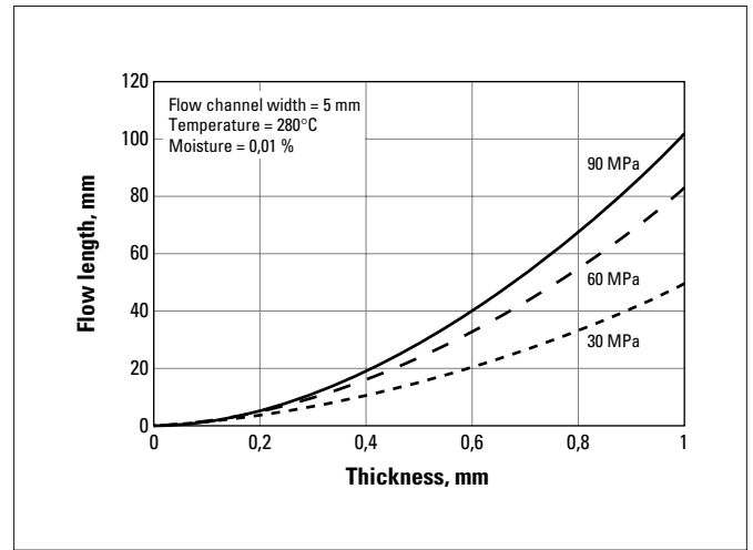
Fig. a.56 RYNITE® 936CS NC010
