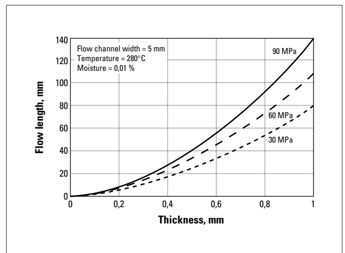
Fig. a.60 RYNITE® FR943 NC010
