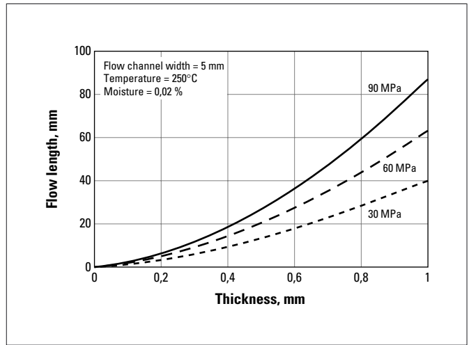
Fig. a.2 CRASTIN® S600F10 NC010
