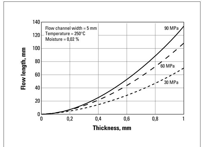
Fig. a.8 CRASTIN® SK602 NC010
