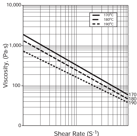
Figure 2. Viscosity/Shear Rate Data
