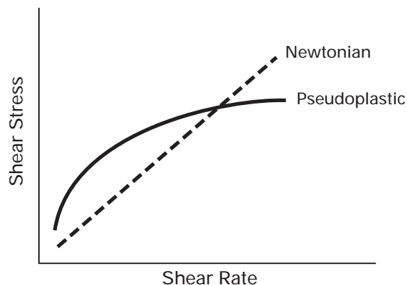
Figure 1. Flow curves for Newtonian and Pseudoplastic Materials.
