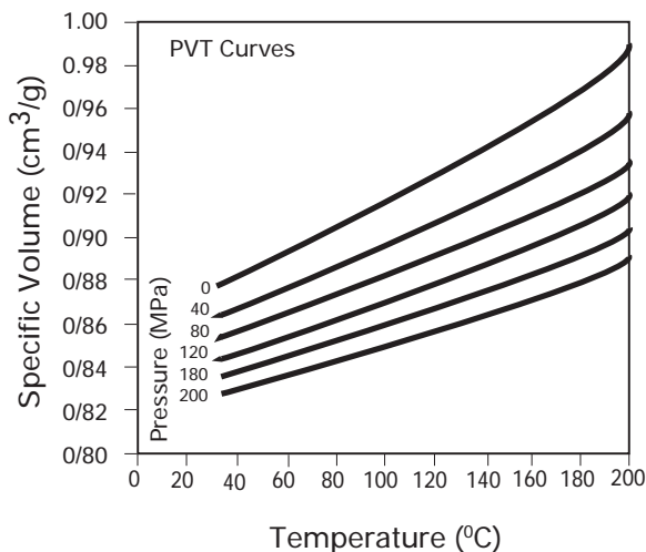
Figure 3. Volume as a Function of Pressure and Temperature
